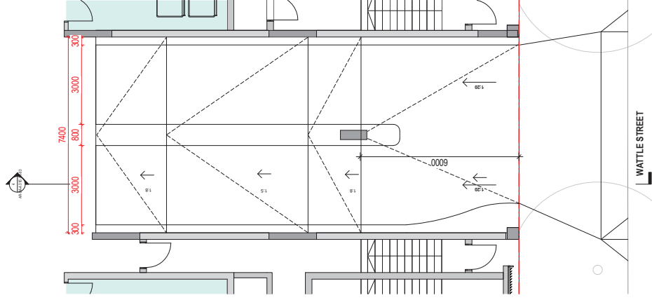
2 CARPARK RAMP LEVEL 01 DOWN TO LEVEL 00
