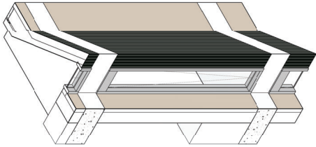
3. PRIVACY DETAIL A - 3D AXONOMETRIC SCALE: 1:20
