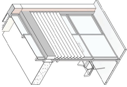
6. PRIVACY DETAIL B - 3D AXONOMETRIC SCALE: 1:20
