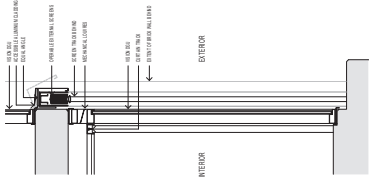
5. PRIVACY DETAIL B - SECTION SCALE: 1:20
